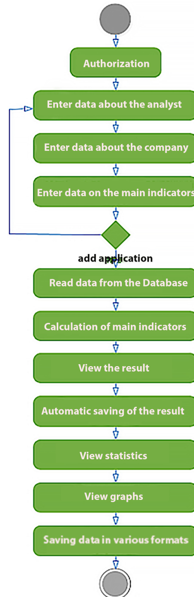
Fig. 1. Diagram of analytics activity
