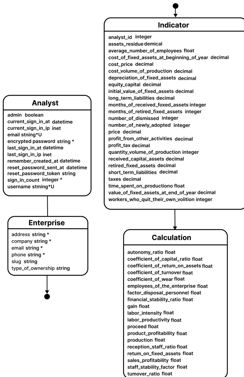
Fig. 3. Database structure
